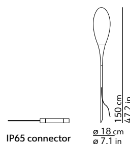
IP65 connector
